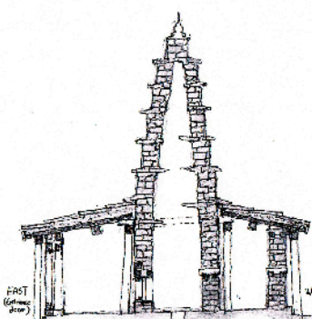
0 1 2 3 4 5m SECTIONS
