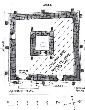
TEMPLE IN SYADA/HUMLA, NEPAL H. WAARHAARD, D. NORLING, OSLO, JUNE - 14.
