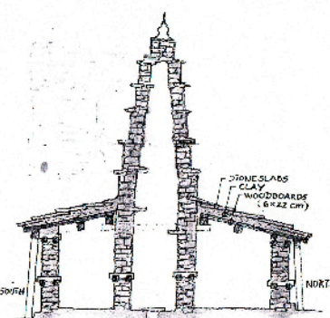
TEMPLE IN SYADA/HUMLA, NEPAL H. WAARHAARD, D. NORLING, OSLO, JUNE - 14.
