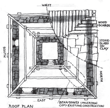
TEMPLE IN SYADA/HUMLA, NEPAL H. WAARHAARD, D. NORLING, OSLO, JUNE - 14.
